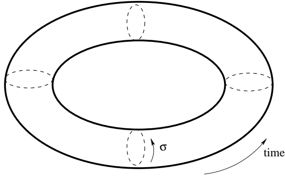
Figure 15: The one-loop closed string vacuum diagram is a two dimensional torus.
