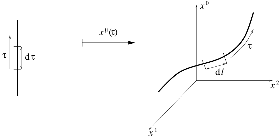
Figure 6: The embedding \tau \mapsto x^\mu(\tau) of a particle trajectory into d -dimensional spacetime. As \tau increases the particle propagates along its one-dimensional worldline in the target space.
