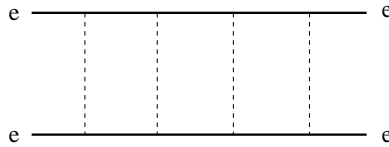
Figure 2: A non-renormalizable ultraviolet divergent Feynman diagram in quantum gravity. The dashed lines depict graviton exchanges.
