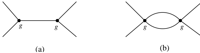
Figure 11: Feynman graphs for four-particle (a) tree-level and (b) one-loop scattering amplitudes in quantum field theory. The lines denote propagators which correspond to the worldlines of particles in spacetime. Each vertex has a coupling constant g associated to it and represents a singular worldline junction responsible for the ultraviolet divergences in loop amplitudes.
